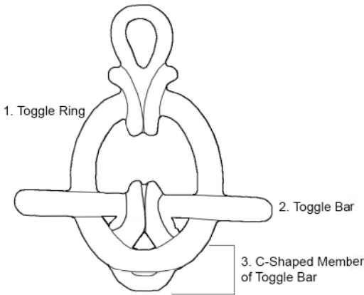
Front View Toggle Clasp
